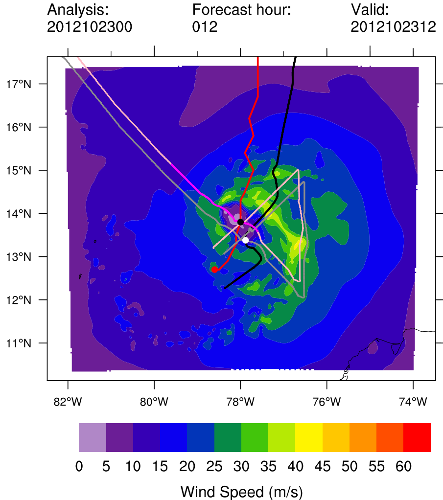
Figure 14: Comparison between the actual flight trajectory in the real Tropical Storm Sandy (grey curves) and the simulated trajectory that has been navigated onto the center of the HWRf-simulated Sandy (pink curves) for the 12-h forecast from the model cycle initialized at 00Z on 23 October 2012. The portions of the trajectory that correspond to the synthetic radial legs are also shown (magenta curves). For reference, the plot also displays the wind center track of the actual storm (black curve), the corresponding track of the HWRf-simulated storm (red curve), the position of the real storm at the analysis time (white dot), the position of the simulated storm at the analysis time (red dot), the position of the real storm at the time slice valid time (white dot), and the position of the simulated storm at the time slice valid time (black dot). The model's simulated wind speed is shown (color contours) at the pressure level nearest that of the average pressure of the first radial leg. While only radial legs whose midpoint times fell within \pm 1.5 h of the model time slice are shown, the full flight trajectories are shown for a time window of \pm 2 h to completely encompass any radial legs near the edge of the time window.
