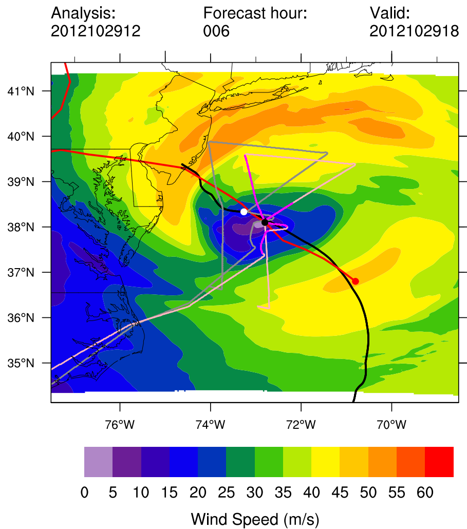
Figure 23: Plan view of synthetic trajectories for the 6-h forecast verifying at 18Z on 29 October 2012. This model cycle was initialized at 12Z on 29 October 2012.
