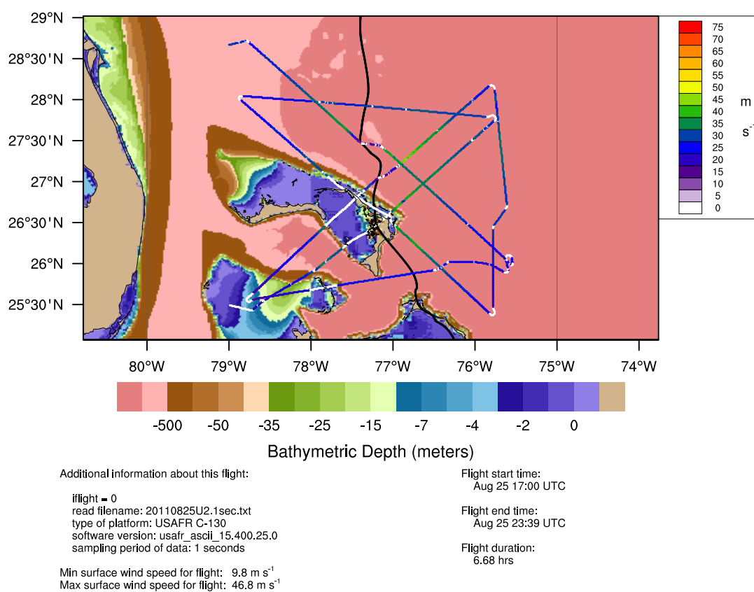
Figure 7: As in Fig. 4, but now showing the SFMR wind speed values that have undergone QC measures to screen out values over land, shallow water, or when the plane was turning rapidly.
