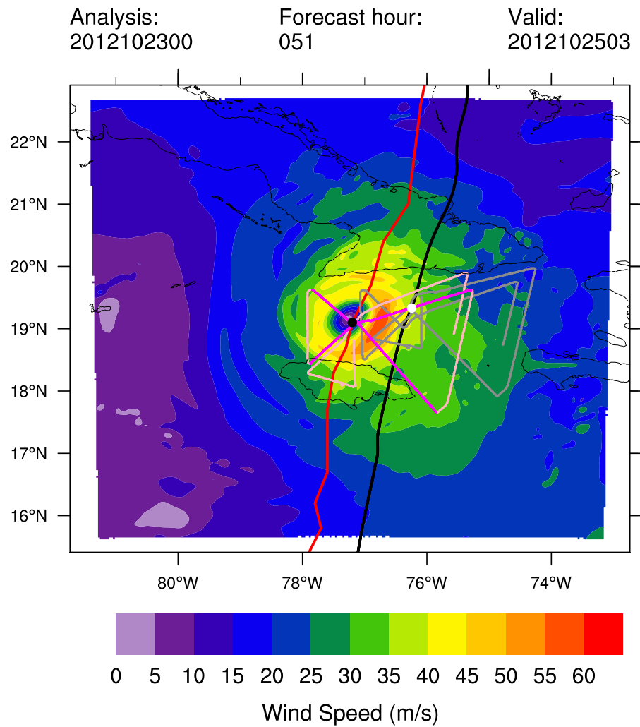
Figure 18: Plan view of synthetic trajectories for the 51-h forecast from the model cycle initialized at 00Z on 23 October 2012.
