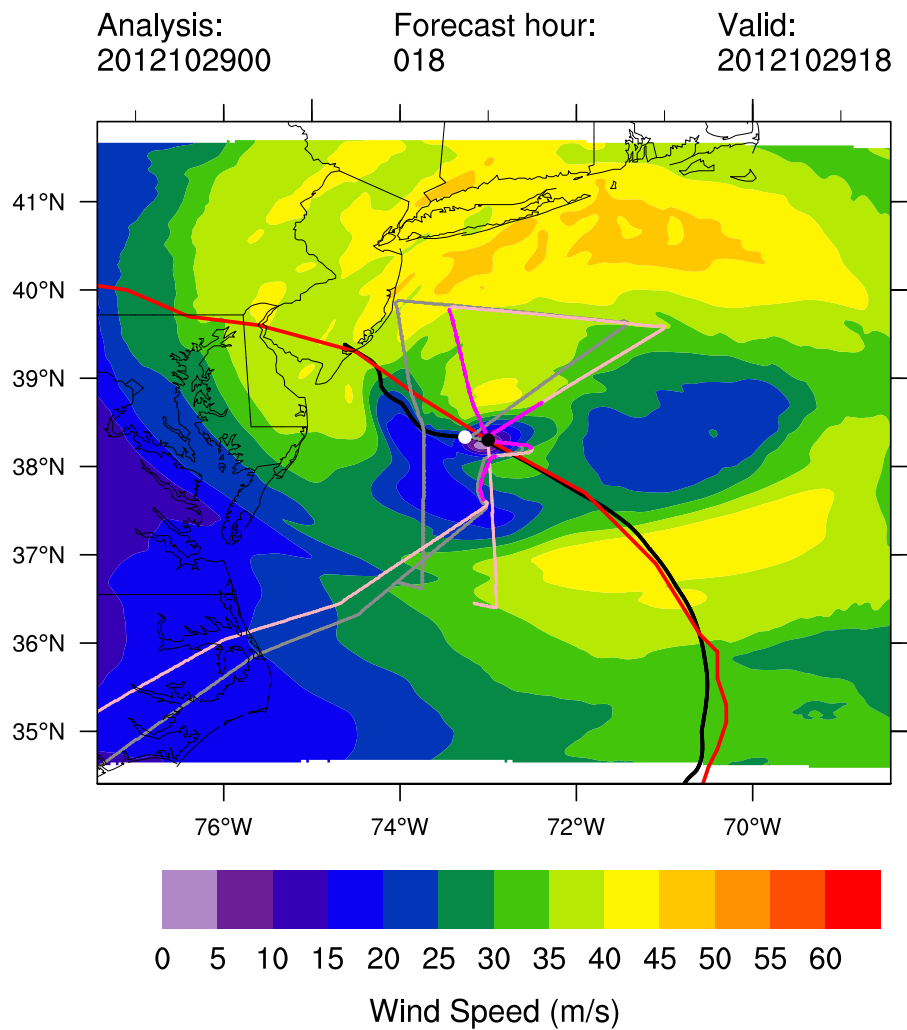
Figure 22: Plan view of synthetic trajectories for the 18-h forecast verifying at 18Z on 29 October 2012. This model cycle was initialized at 00Z on 29 October 2012.
