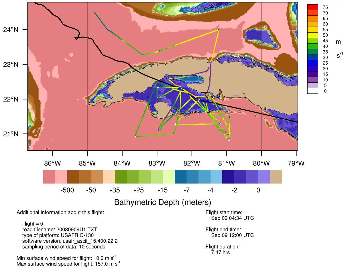
Figure 2: Retrieved SFMR surface wind speeds without any additional quality control measures (lines colored by retrieved wind speed) plotted atop bathymetric depths (color shading) from the ETOPO1 data set for Ike (2008). Note that the scale for bathymetric is highly nonlinear in order to emphasize gradients in shallow water. The black line shows the track of the storm, as determined by wind centers obtained from the Willoughby-Chelmon center finding method.
