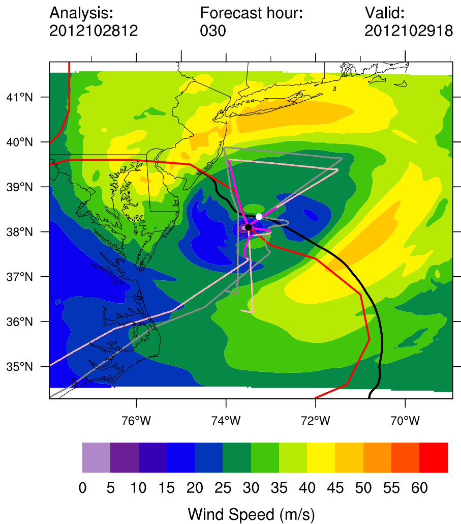
Figure 21: Plan view of synthetic trajectories for the 30-h forecast verifying at 18Z on 29 October 2012. This model cycle was initialized at 12Z on 28 October 2012.
