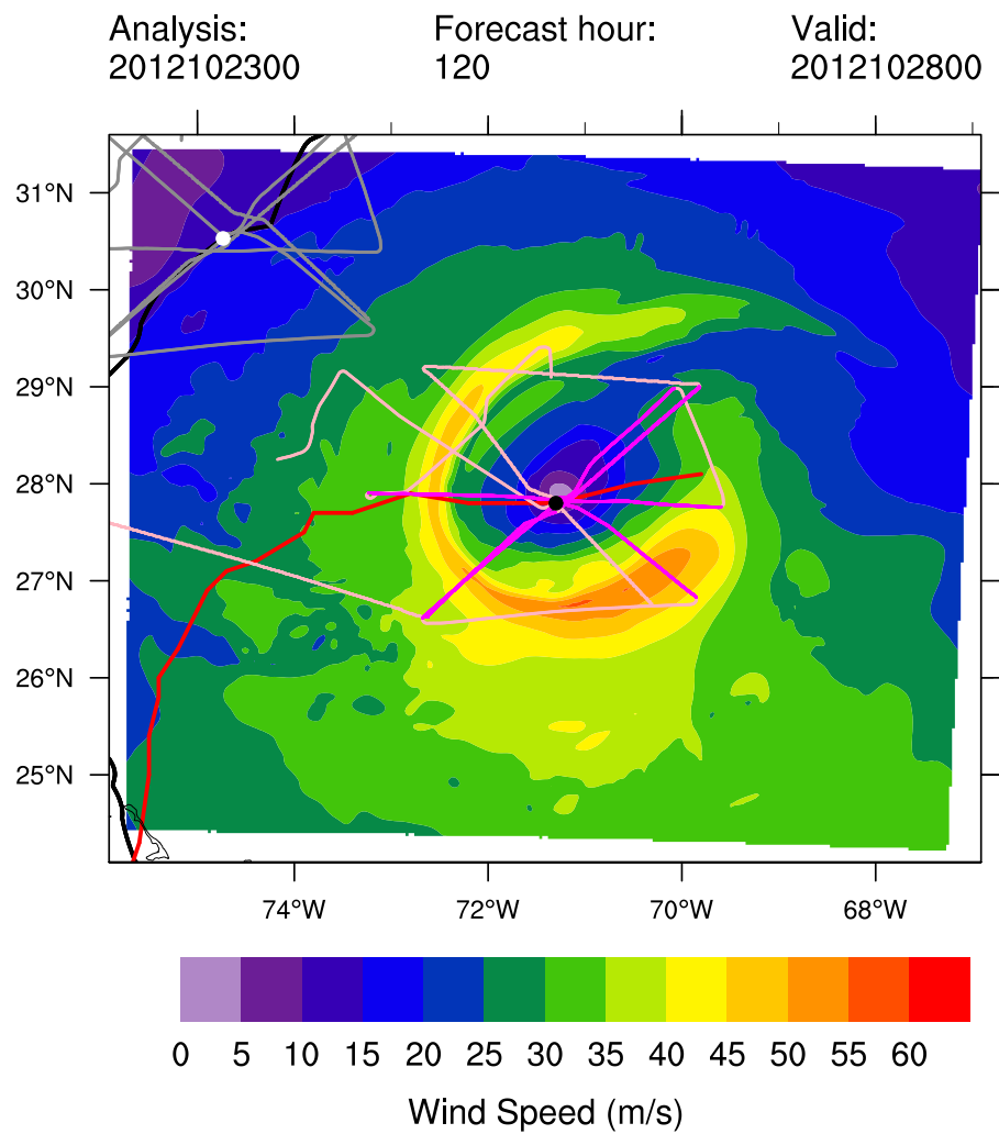
Figure 19: Plan view of synthetic trajectories for the 120-h forecast from the model cycle initialized at 00Z on 23 October 2012.
