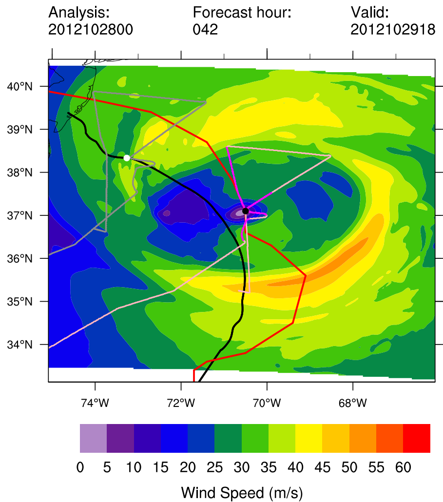
Figure 20: Plan view of synthetic trajectories for the 42-h forecast verifying at 18Z on 29 October 2012. This model cycle was initialized at 00Z on 28 October 2012.
